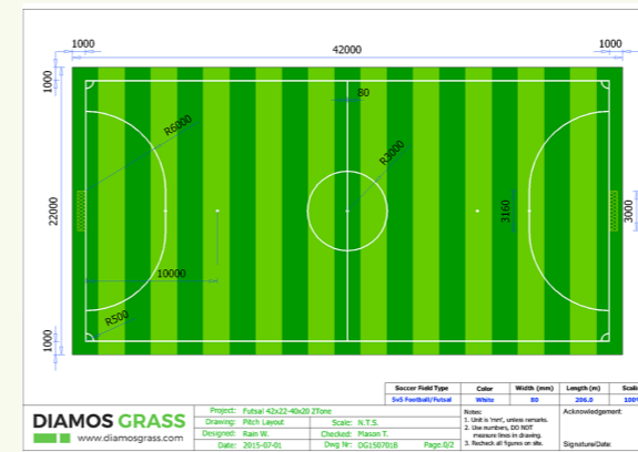
Futsal 42x22-40x20 2Tone Green
