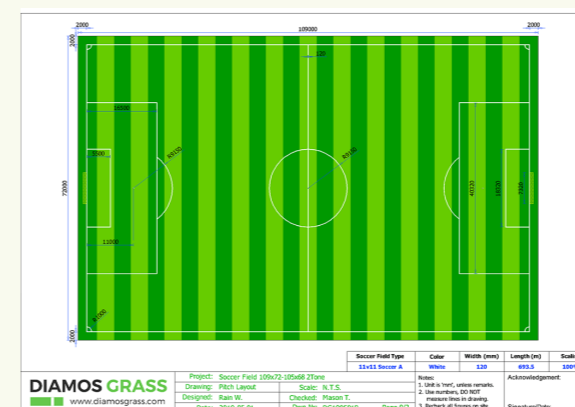
11v11 Soccer 109x72-105x68 2Tone
