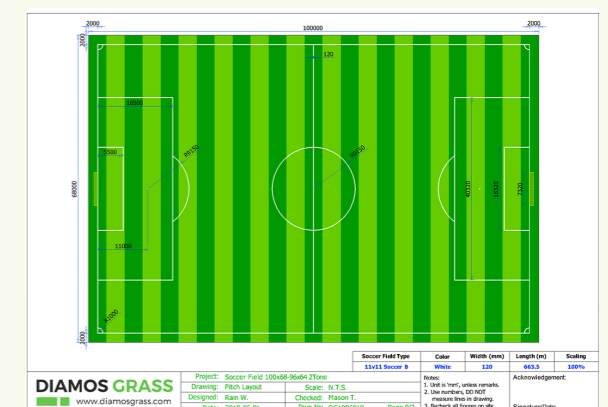
11v11 Soccer 100x68-96x64 2Tone
