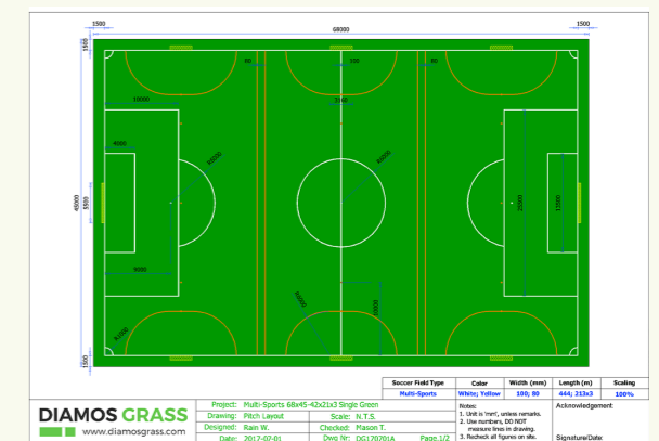
Multi-Sports 68x45-42x21x3 Single
